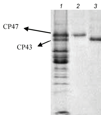
Fig. 1. Electrophoretic pattern of purified CP43 and CP47 in 15 % acrylamide gel containing 6 M urea. Lanes 1, 2, and 3 are for photosystem 2, CP47, and CP43, respectively. Proteins were stained with Coomassie brilliant blue R-250.
